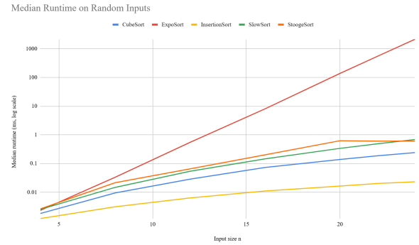
Fig. 1. Median runtime on random inputs across 101 trials. The y-axis is logarithmic because ExpoSort grows much more quickly than the comparison algorithms.
